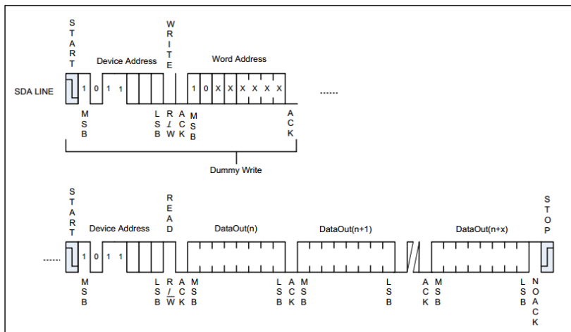
Figure 11 Sequential Read
