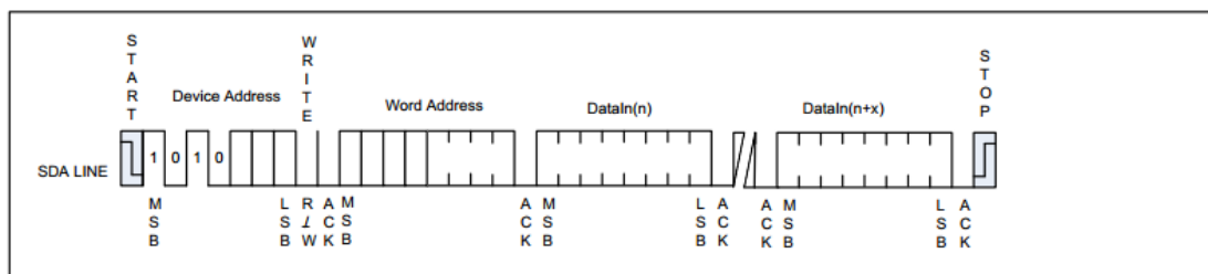
Figure 6 Page Write
