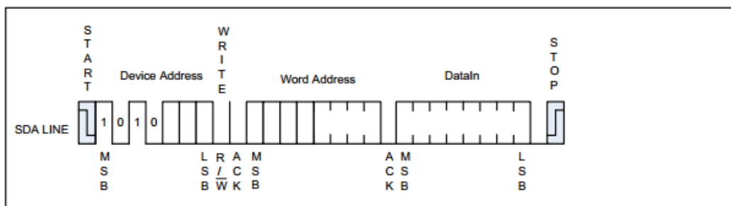
Figure 5 Byte Write
