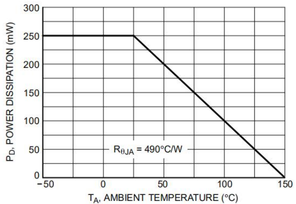
Figure 06. Derating Curve
